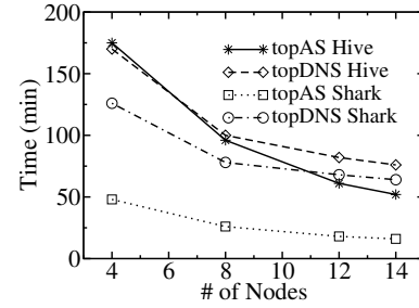
Figure 5: Nodes Scalability.
