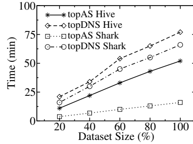
Figure 4: Dataset Scalability.
