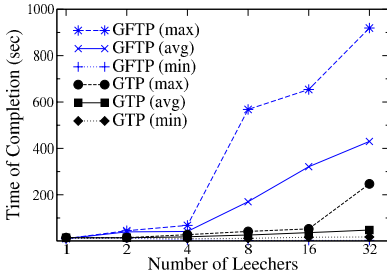
Fig. 8. Min, max and average time of completion for both GridFTP and GTP over various number of downloaders in the WAN setting
