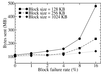
Fig. 5. Average size of uploaded data from leechers only over various number of failure rates and block sizes
