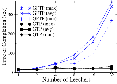
Fig. 6. Min, max and average time of completion for both GridFTP and GTP over various number of downloaders in the LAN setting
